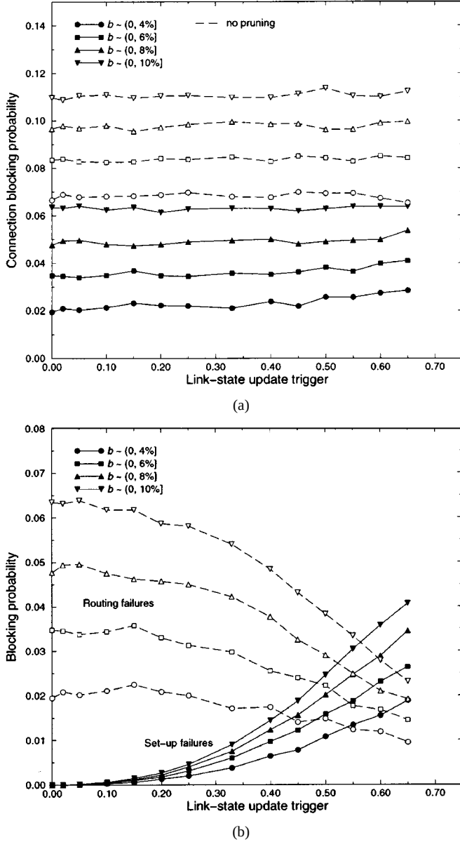
Fig. 4. Blocking insensitivity to triggers: Connection blocking remains fairly constant over a wide range of link-state update triggers, with and without pruning enabled. Across the four curves for different bandwidth ranges, the mean connection holding time \ell is varied to keep the offered load constant. The experiments evaluate the MCI topology with \rho = 0.70 , \lambda = 1 , and \alpha = 1 . The mean connection durations are 50.4, 33.6, 25.2, and 20.2 for the mean bandwidths 2%, 3%, 4%, and 5%, respectively.
