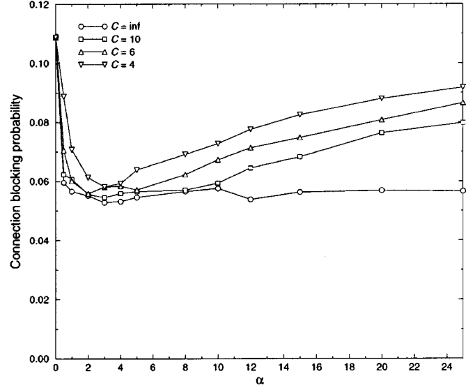
Fig. 9. Exponent \alpha with stale link-state information: A larger exponent \alpha decreases the blocking probability, until \alpha grows so large that the cost intervals become too narrow. This experiment evaluates the random topology with update period = 10, \rho = 0.75 , \lambda = 1 , b \sim (0.0, 0.06] , \ell = 40.6 , and pruning disabled.
