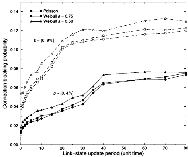
Fig. 2. Blocking for varying arrival burstiness: Burstiness is increased with a smaller Weibull shape parameter, a . Simulation parameters are the same as in Fig. 1(a).
