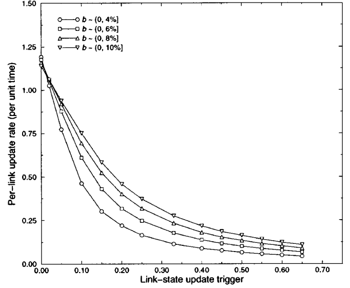
Fig. 5. Link-state update rate for different trigger values: This graph shows the link-state update rate for the random topology with \rho = 0.75 , \lambda = 1 , \alpha = 1 , and pruning disabled. Mean connection durations are the same as in Fig. 1.
