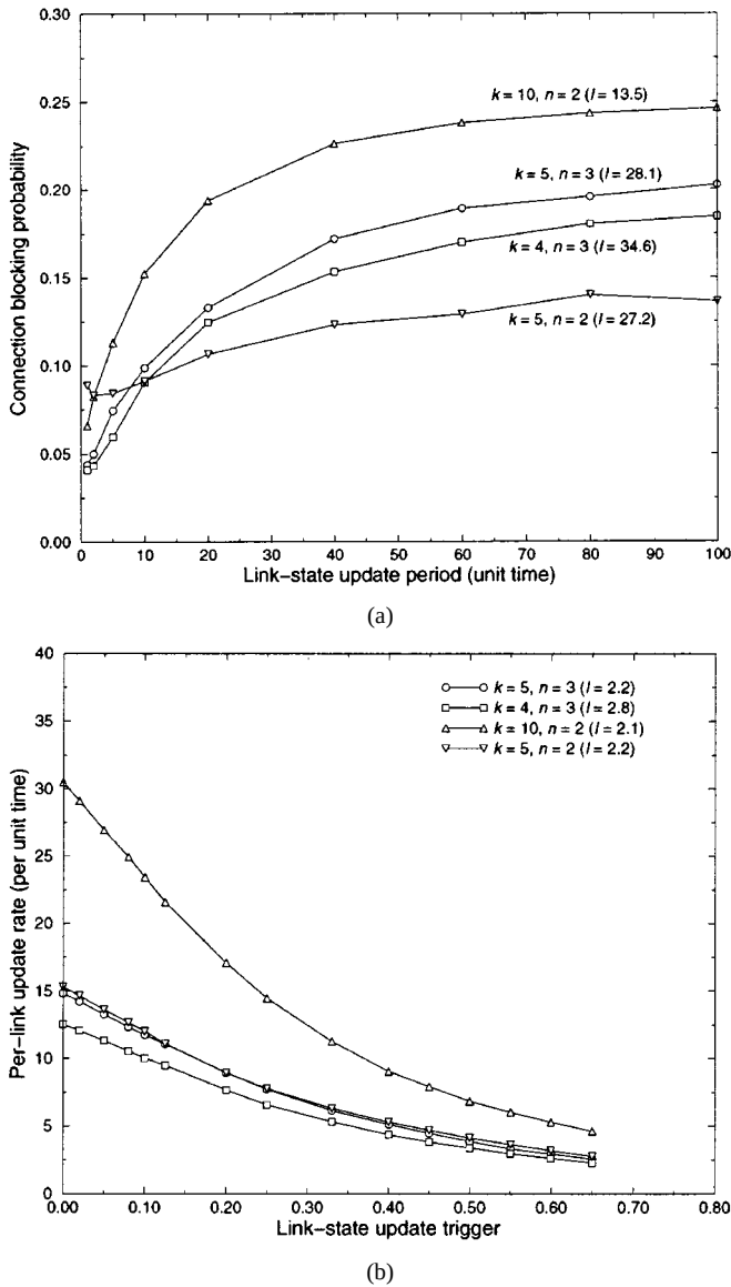
Fig. 7. Topology and link-state accuracy: (a) Richly connected topologies have low blocking probabilities under accurate information, although the benefits of multiple routes degrade under large update periods. (b) With triggered updates, the rate of link-state messages is proportional to k and independent of n . In both experiments, \rho = 85\% , b \sim (0, 0.1] , and \alpha = 2 (with pruning). The arrival rates in both graphs are \lambda = 1 and \lambda = 12.5 , respectively. Load is kept constant across the four topologies by changing \ell .
