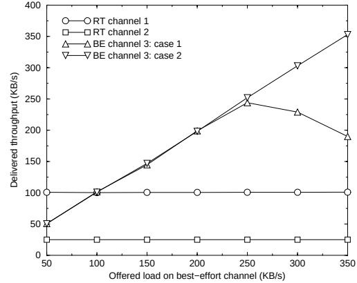
Figure 6. Channels 1 and 2 have the same parameters as in Figure 5(b) but channel 1 underutilizes its reservation. In case 1, channel 1 generates 20 KB messages at 5 msg/s; in case 2, it generates 10 KB messages at 10 msg/s.
