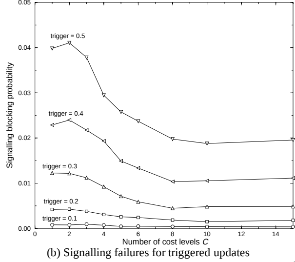
Figure 4. Discretized costs with stale link-state information: Both experiments simulate the 5-ary 3-cube with \rho = 0.85 , b \sim (0.0, 0.1] , \lambda = 1 , \ell is exponentially distributed with mean 28, and \alpha = 1 .
